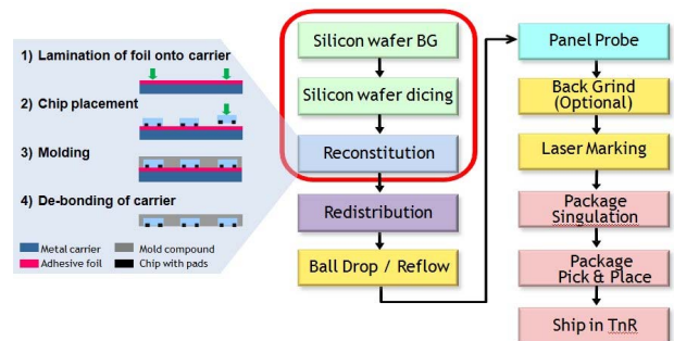
Figure 2. eWLB Assembly Process Flow
