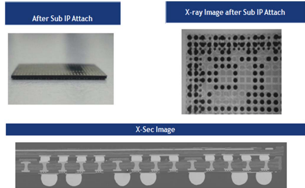
Figure 8. Micrographs of 3D eWLB SiP with interposer
