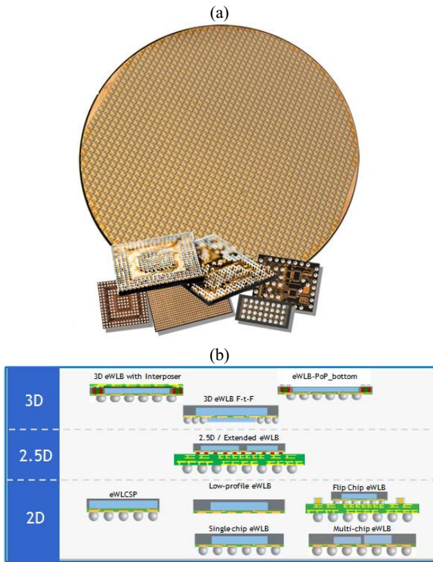
Figure 1. (a) 300mm eWLB carrier and eWLB packages, and (b) evolution of eWLB technology from 2D to 2.5D/3D packaging solution
