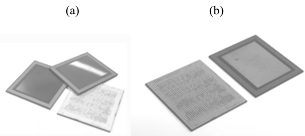
Figure 4. Micrograph of 3D eWLB-PoP; (a) TV1 and (b) TV2 Component Level Reliability of 3D eWLB-PoP
